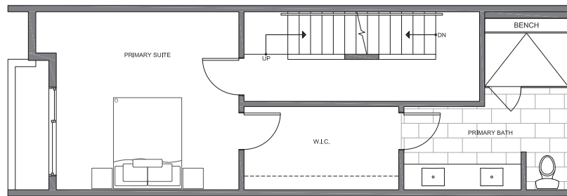
THIRD FLOOR
