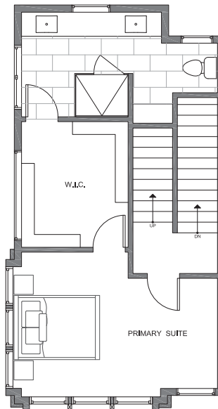
THIRD FLOOR
