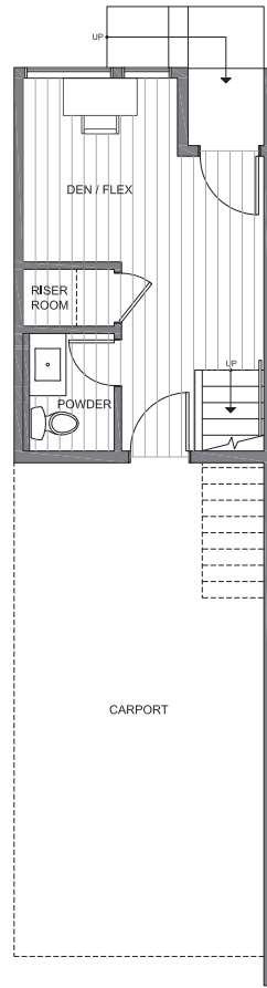
FIRST FLOOR
