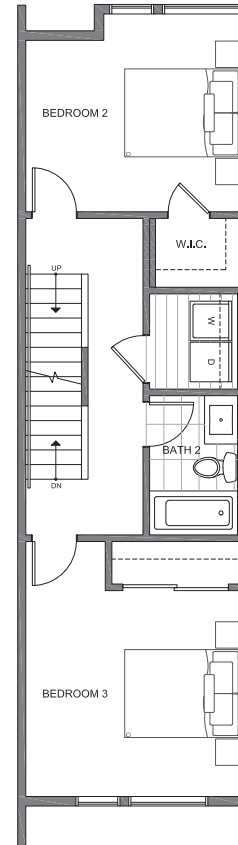
THIRD FLOOR
