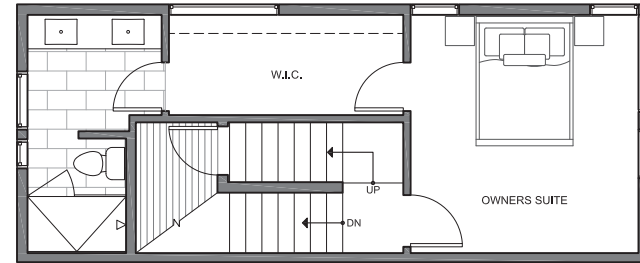
THIRD FLOOR
