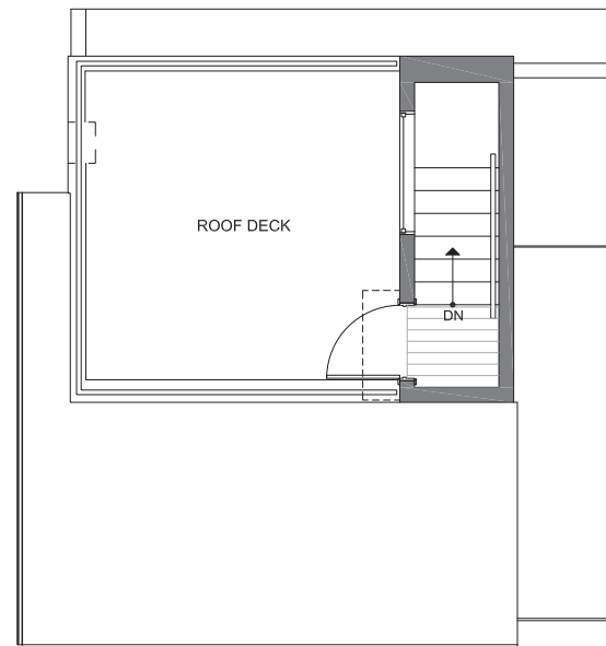
ROOF DECK
