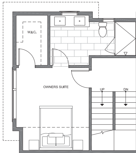
THIRD FLOOR
