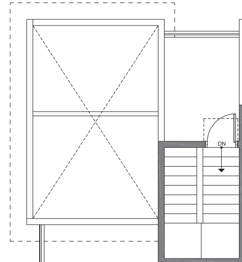
ROOF DECK
